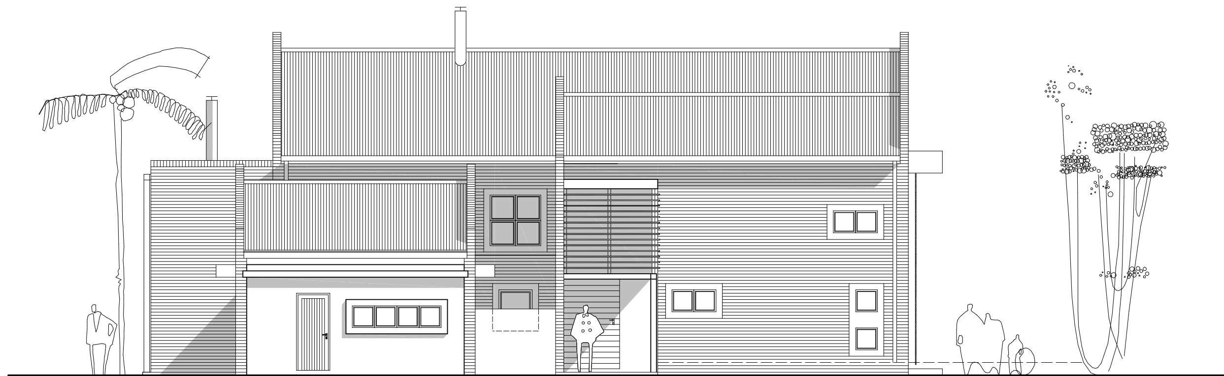
SOUTH Elevation
